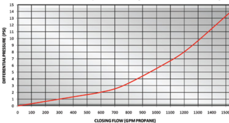
4" Internal Valve Liquid LPG Closing Flow-Downward Discharge
